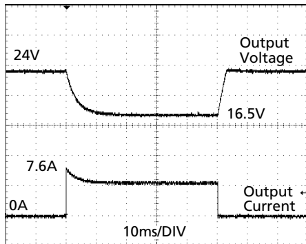
Fig. 21-1 7.6A peak current for 50ms , typ. (2x the nominal current)
